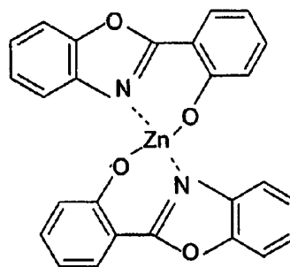
ZnPBO
