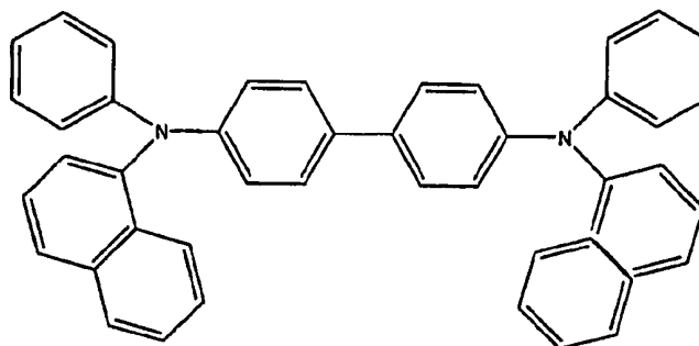
\beta -NPD
