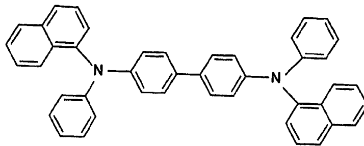
\alpha -NPB
